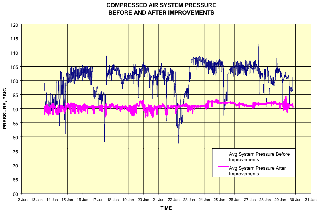
Figure 1. Compressed Air Power Before and After Improvements
